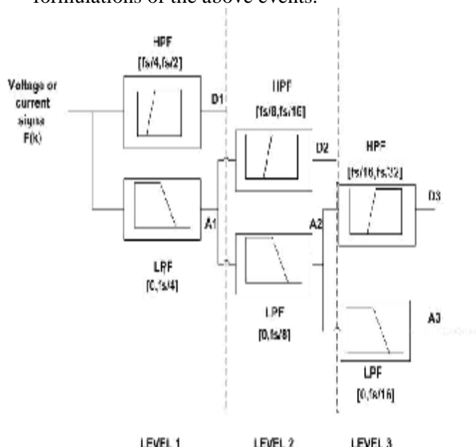
Figure. 7. Algorithm for DWT coefficient decomposition *HPF: High Pass Filter **LPF: Low Pass Filter
