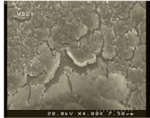
Figure 4. SEM image of silicon surface after battery test.
