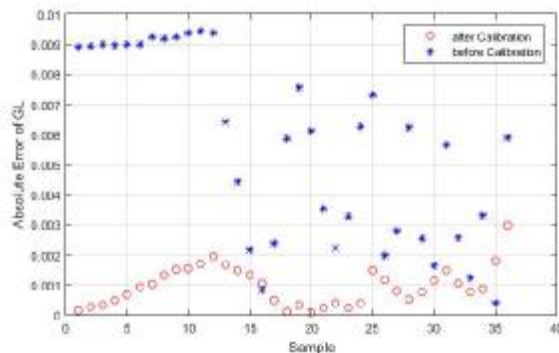
Figure 7. Absolute Error of GL, before and after 30 parameters calibration
