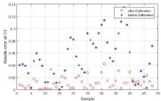
Figure 6. Absolute Error of Tilt angle, before and after 12 parameters calibration
