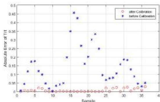
Figure 8. Absolute Error of Tilt angle, before and after 30 parameters calibration
