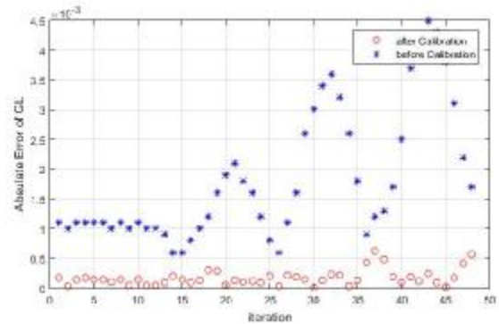
Figure 5. Absolute Error of GL, before and after 12 parameters calibration
