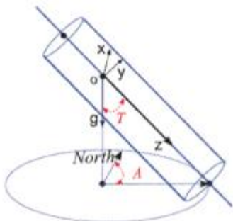
Figure 3. Tilt and azimuth angles [2]
