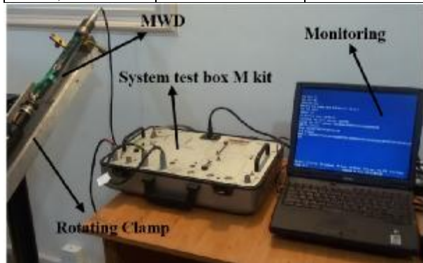
Figure 4. MWD instrument and calibration tools
