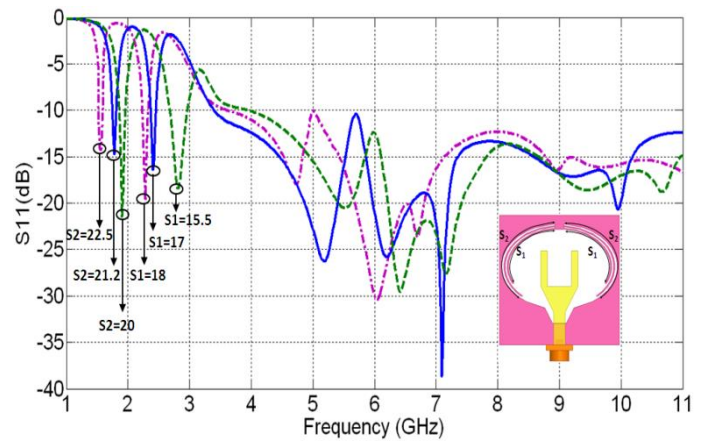
Fig. 4. Simulation results for reflection coefficients of the proposed antenna for different values of S1 and S2; these parameters are used for length of edges of inverted U-shaped strip. Other values of this simulation are shown in Table I. The inset shows the antenna structure.
