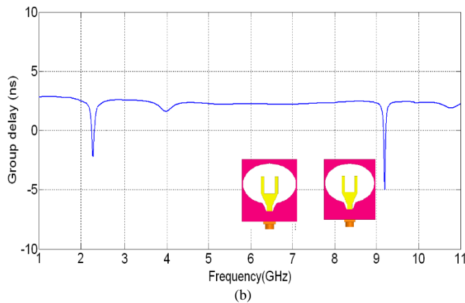
Fig. 9. Simulation results for group delay of the proposed antenna, (a) face-to-face and (b) side-by-side configurations.
