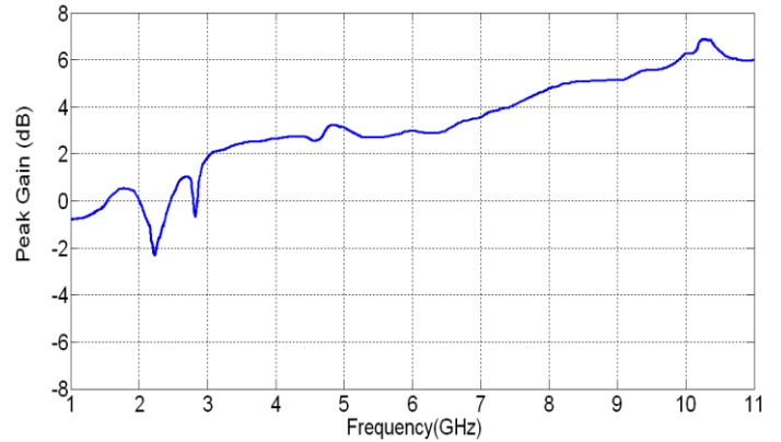
Fig. 8. Measured peak gain of the proposed antenna.
